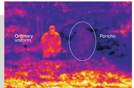
Thermal image 8-12µm, distance 25 m
